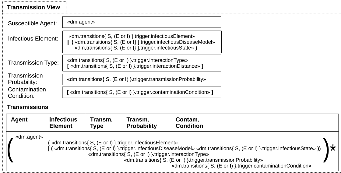
Figure 4.8: Concrete Syntax: Disease Transmission View
