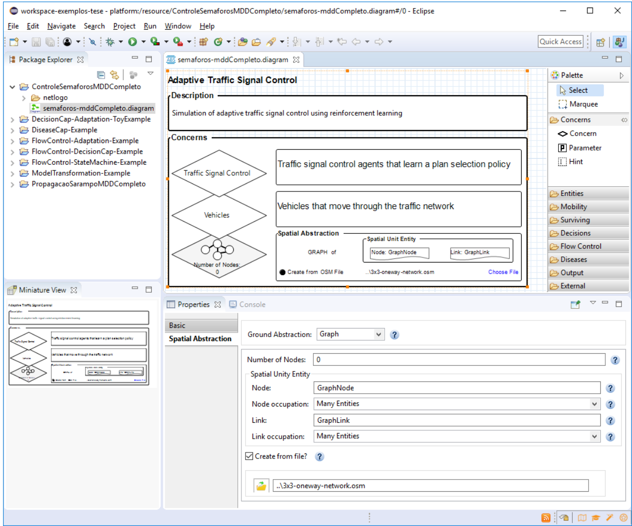
Figure 4.9: ABSTRACTME Tool: User Interface and Overview Diagram
