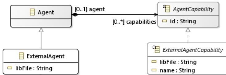
Figure 3.8: Core Metamodel: External Agent and Agent Capability
