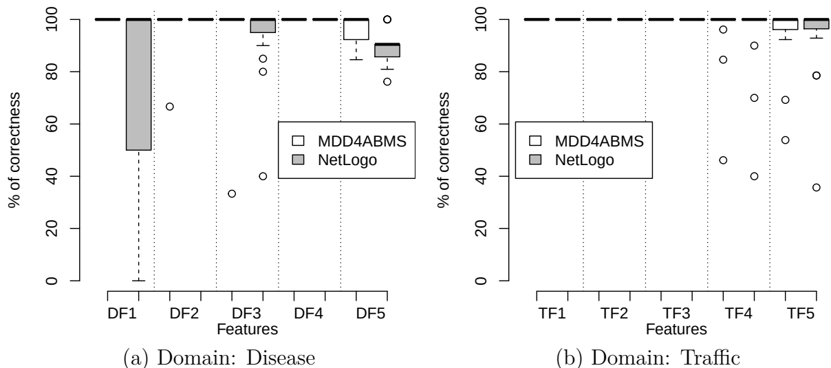
Figure 5.6: Percentage of Correctness of Features
