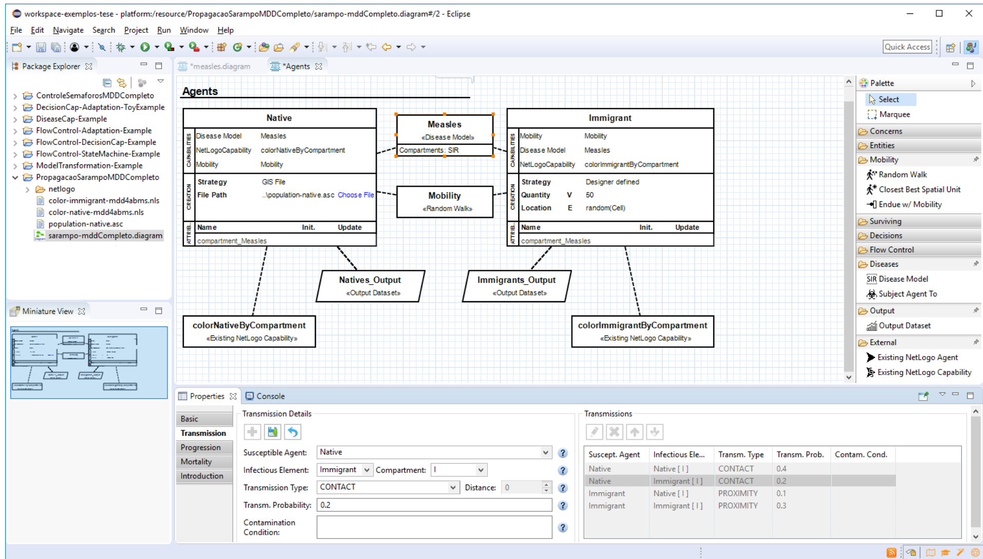
Figure 4.11: ABSTRACTme Tool: Disease Model, Mobility, Output, and External Agent Capability
