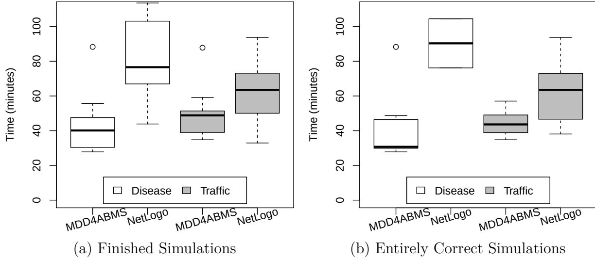
Figure 5.7: Time to Develop Simulations
