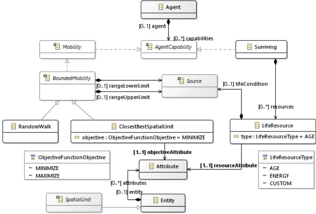
Figure 3.7: Core Metamodel: Mobility and Surviving Agent Capabilities
