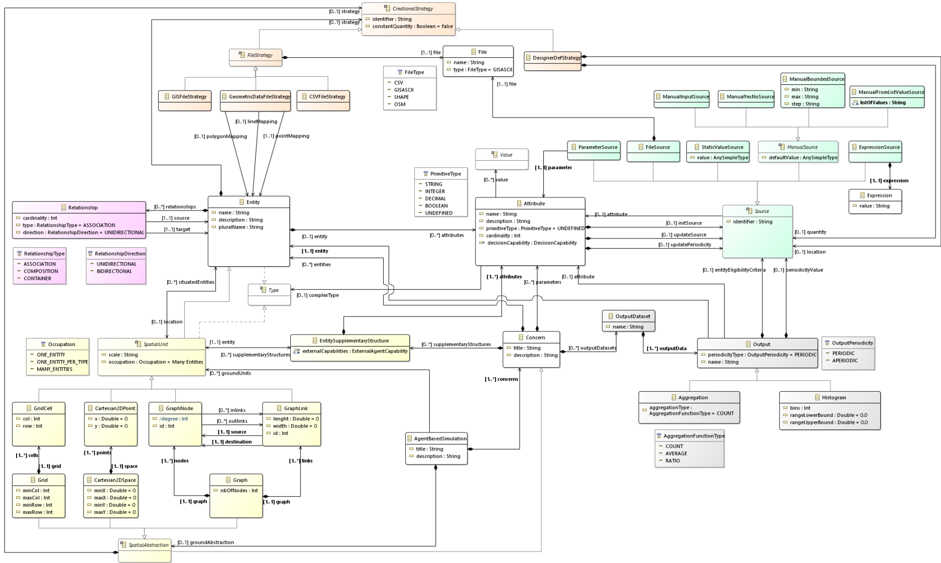
Figure B.1: Complete MDD4ABMS Metamodel: Part 1
