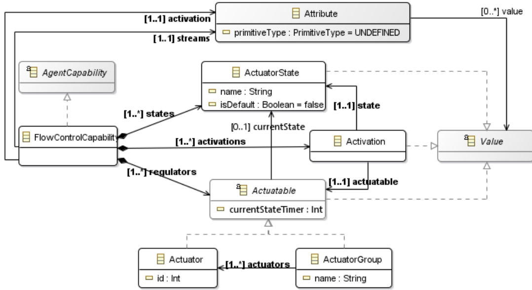
Figure 3.10: Traffic Signal Control Metamodel Extension: Flow Control
