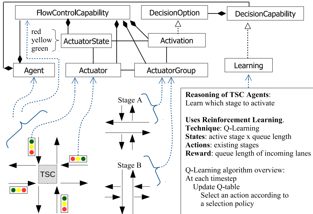
Figure 3.11: Traffic Signal Control: Example of Concept Abstractions
