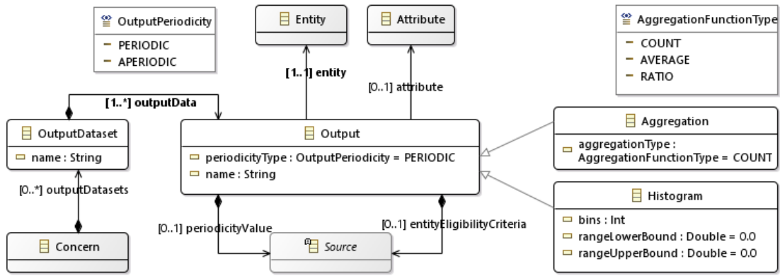
Figure 3.6: Core Metamodel: Simulation Outputs
