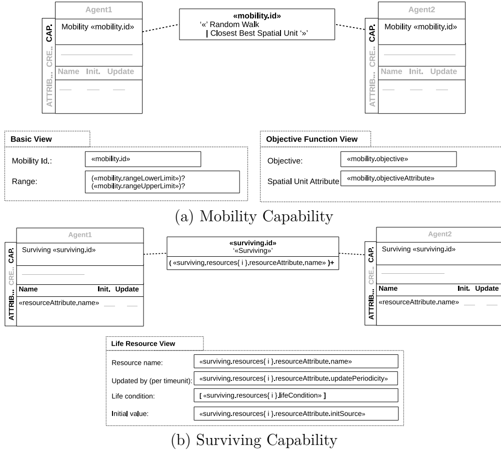
Figure 4.4: Concrete Syntax: Mobility and Surviving Capabilities
