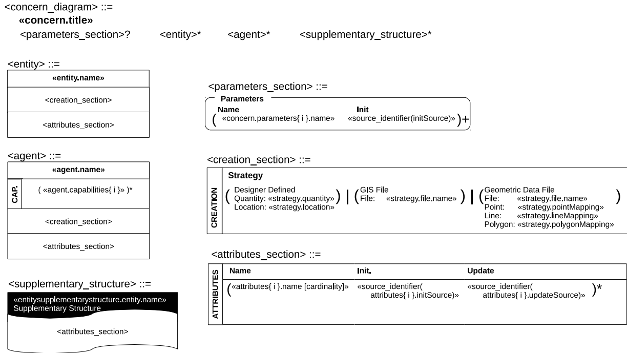
Figure 4.2: Concrete Syntax: Concern, Parameter, Entities, and Agents
