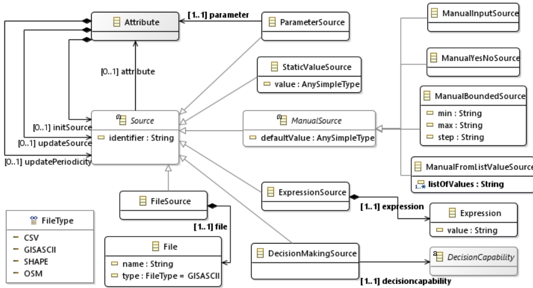
Figure 3.4: Core Metamodel: Sources
