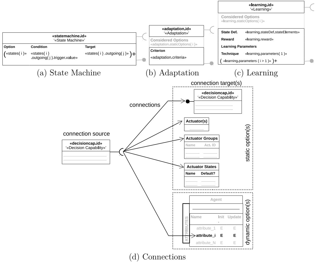
Figure 4.6: Concrete Syntax: Decision Capabilities
