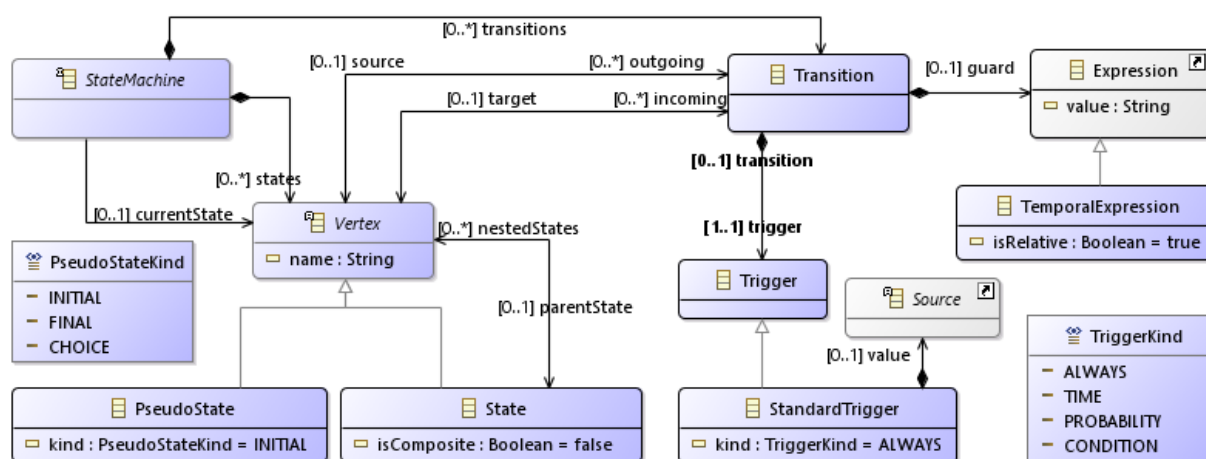
Figure A.1: Abstract State Machine Metamodel
