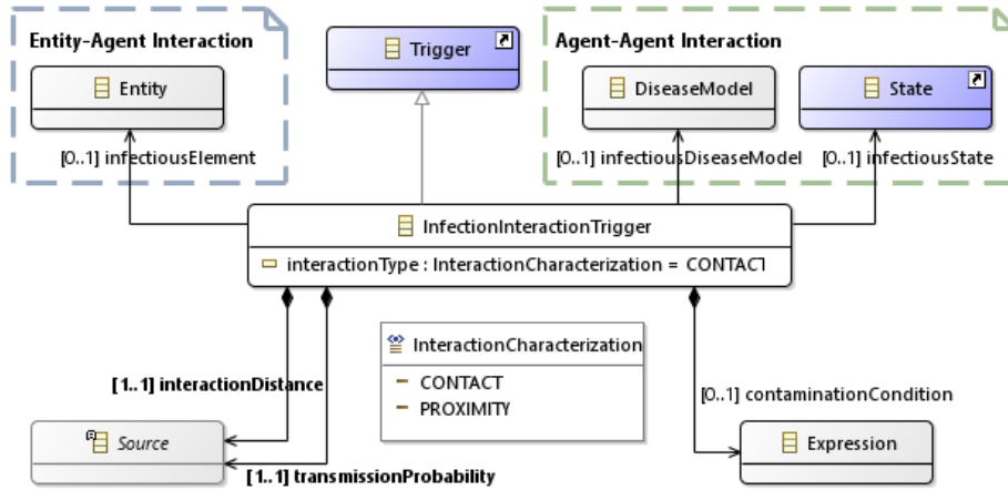
Figure 3.15: Spread of Disease Metamodel Extension: Infection
