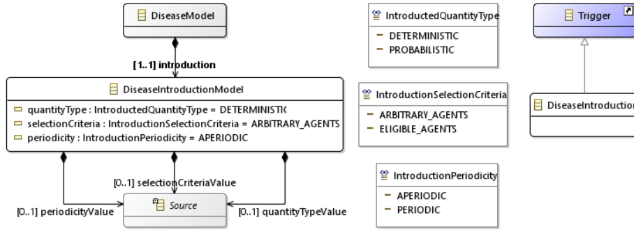
Figure 3.17: Spread of Disease Metamodel Extension: Disease Introduction
