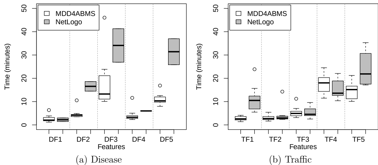
Figure 5.8: Time to Develop Features in Entirely Correct Simulations
