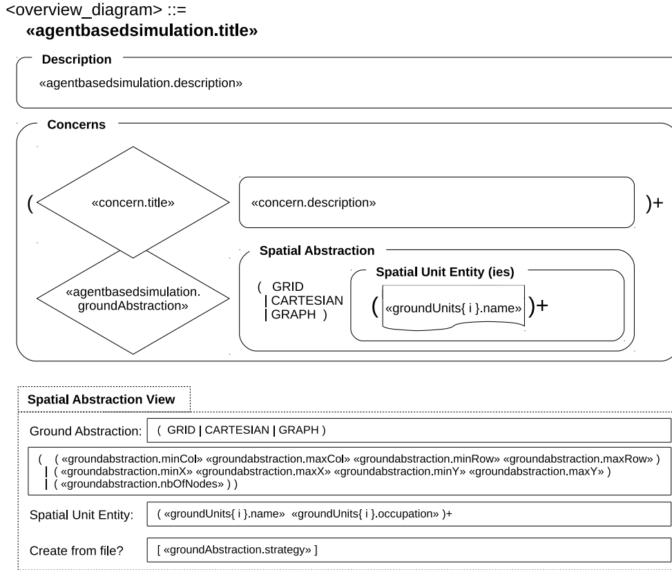
Figure 4.1: Concrete Syntax: Overview Diagram
