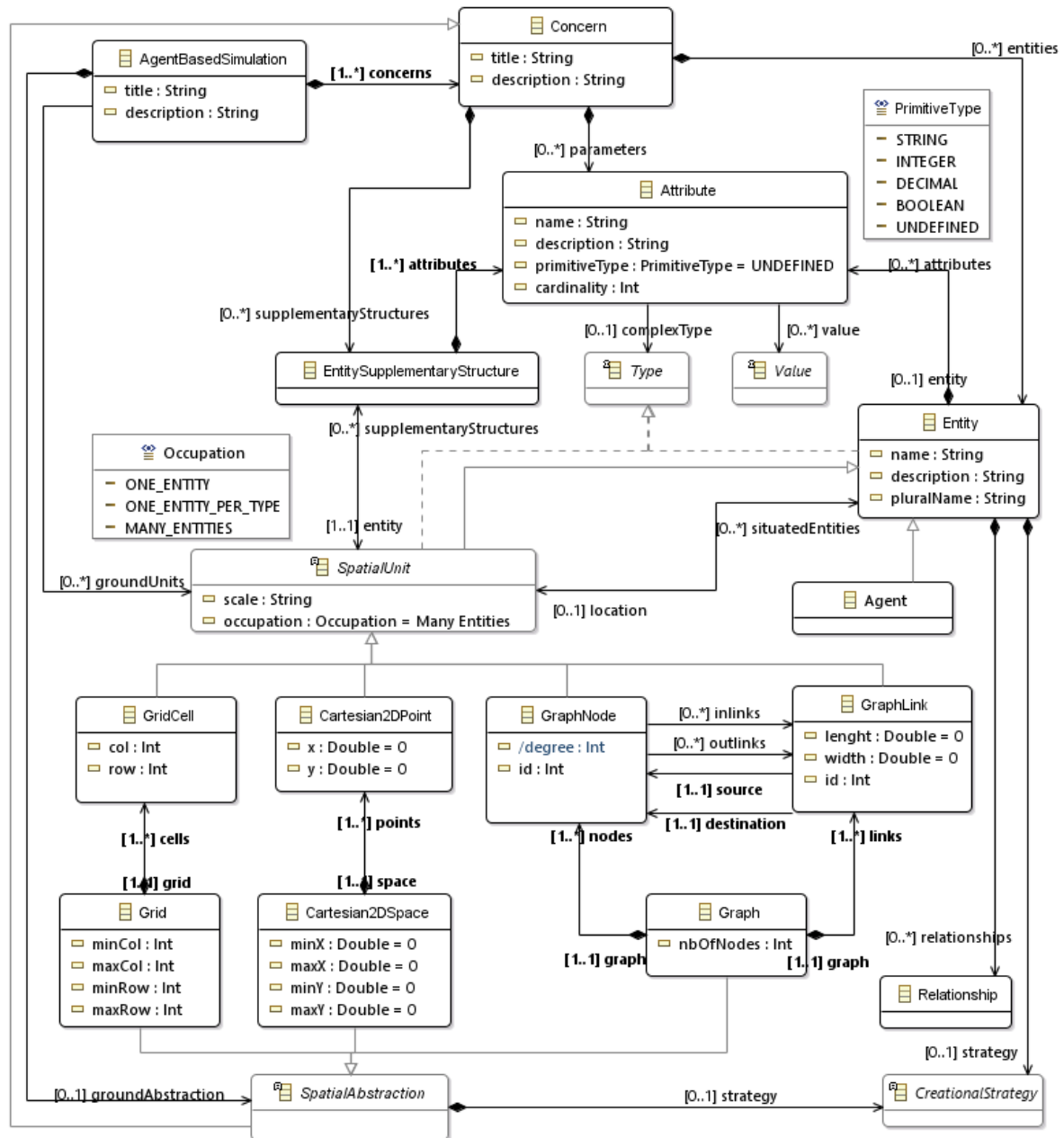
Figure 3.2: Core Metamodel: Environment, Entities, and Agents
