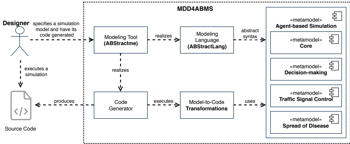
Figure 3.1: Overview of the MDD4ABMS Approach
