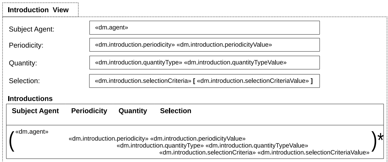
Figure C.3: Concrete Syntax of Disease Elements: Introduction View
