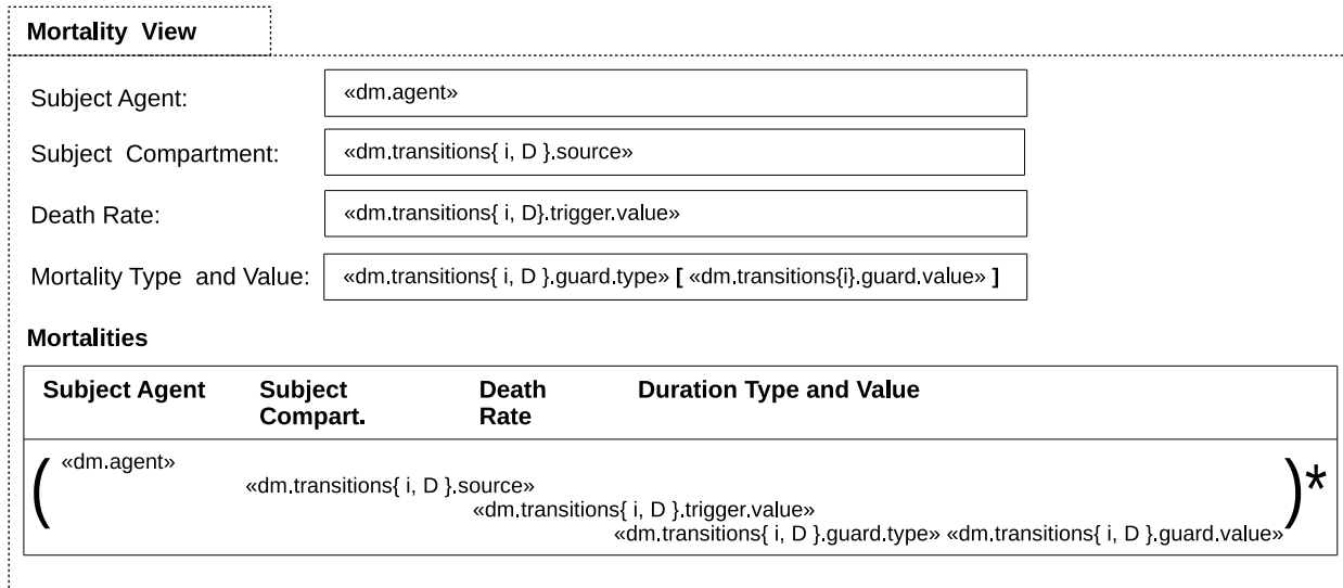
Figure C.2: Concrete Syntax of Disease Elements: Mortality View
