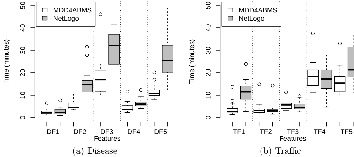
Figure 5.10: Time to Develop Features Considering Finished Simulations
