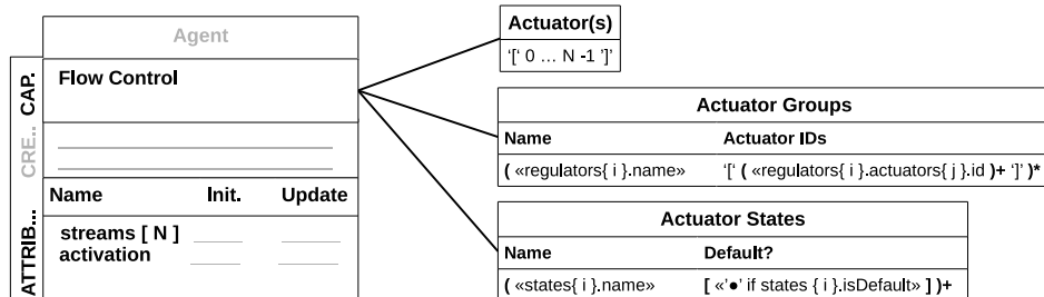
Figure 4.5: Concrete Syntax: Flow Control Capability
