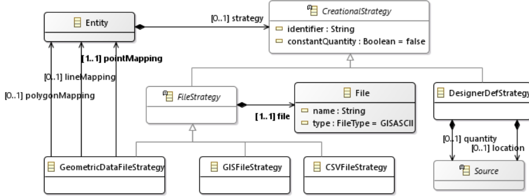
Figure 3.5: Core Metamodel: Creational Strategies
