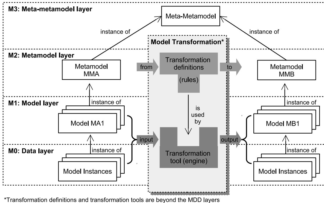
Figure 2.2: MDD Abstraction Layers and Model Transformation Elements. Adapted from Bocciarelli and D’Ambrogio [16]
